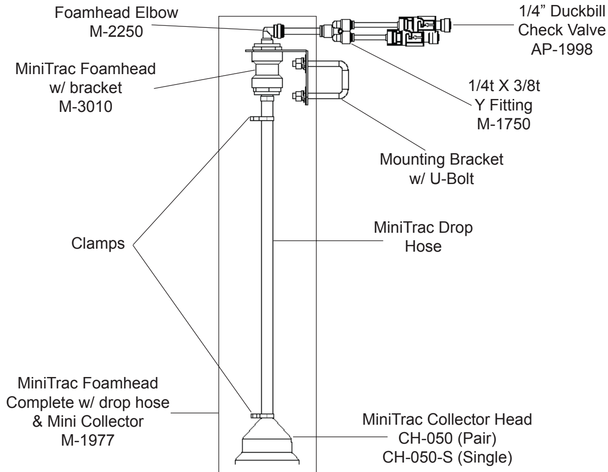
FIGURE 2 - MiniTrac Foamhead and Boom End Assembly
